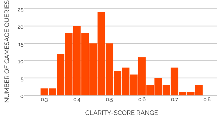
Figure 3: Distribution of clarity scores for the GameSage queries submitted during our experiment ( M = 0.5 , \sigma = 0.11 ). A clarity score for a query is its average cosine similarity relative to the fifty most related games provided for it by GameNet.
