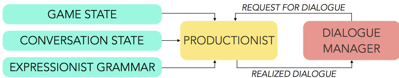
Figure 1: Our NLG architecture. The Productionist module satisfies targeted requests made by our game’s dialogue manager by operating over the game state, conversation state, and an Expressionist grammar to produce fully realized dialogue.
