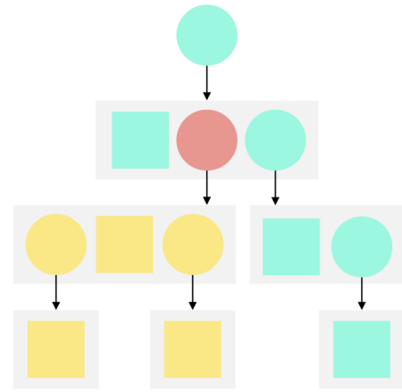
Figure 2: Dialogue production, illustrated. A nonterminal symbol with the desired markup (red) is targeted, triggering production rules (gray)—whose bodies contain terminal (square) and nonterminal symbols (circle)—by both forward chaining (yellow) and backward chaining (aqua). The resulting production (a complete line of dialogue) is the concatenation of the six terminal symbols, and comes packaged with all the markup attributed to the six nonterminal symbols.
